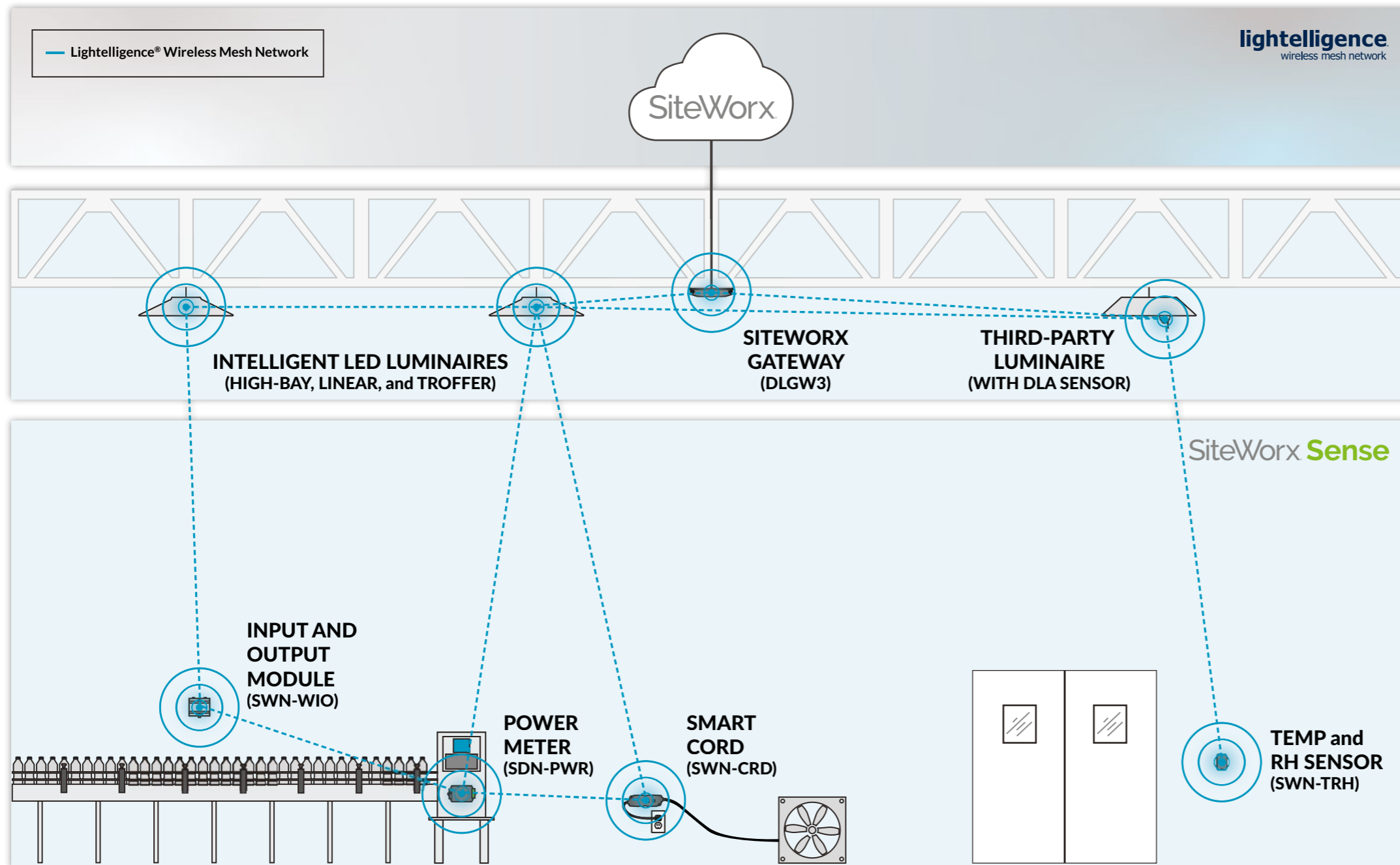
Wireless sensors and meters transmit important facility data such as temperature, humidity, pressure, vibration, flow rate, and power characteristics to SiteWorx using the Lightelligence Wireless Mesh Network.
