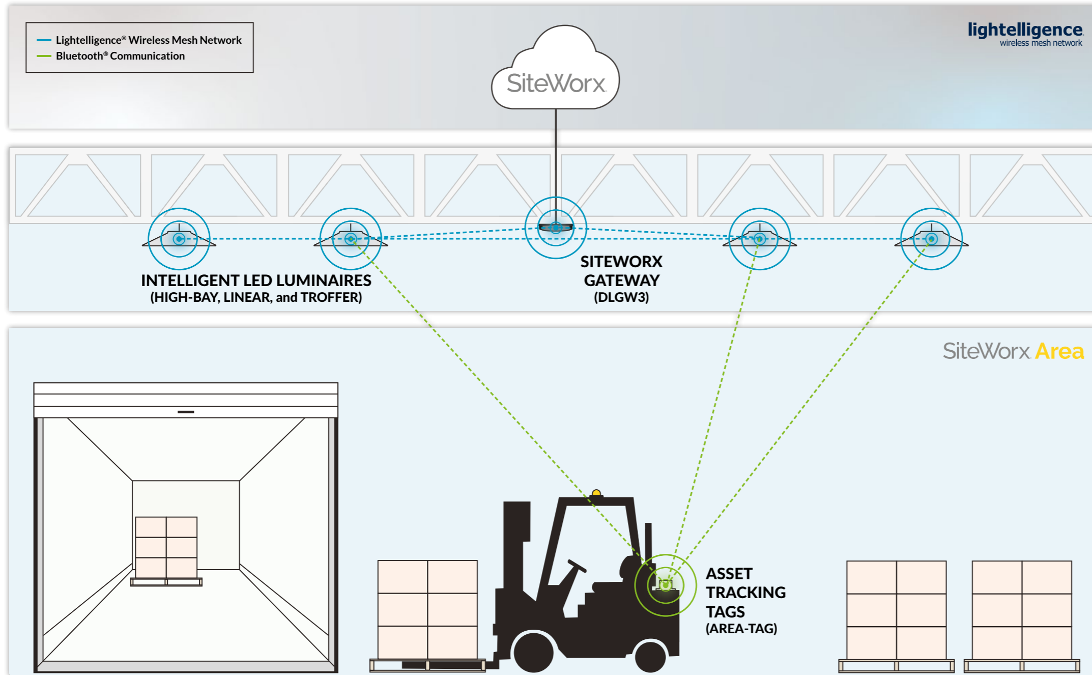
Asset Tracking Tags can be easily deployed to help locate critical equipment or important tools that are constantly moving around your facility.
